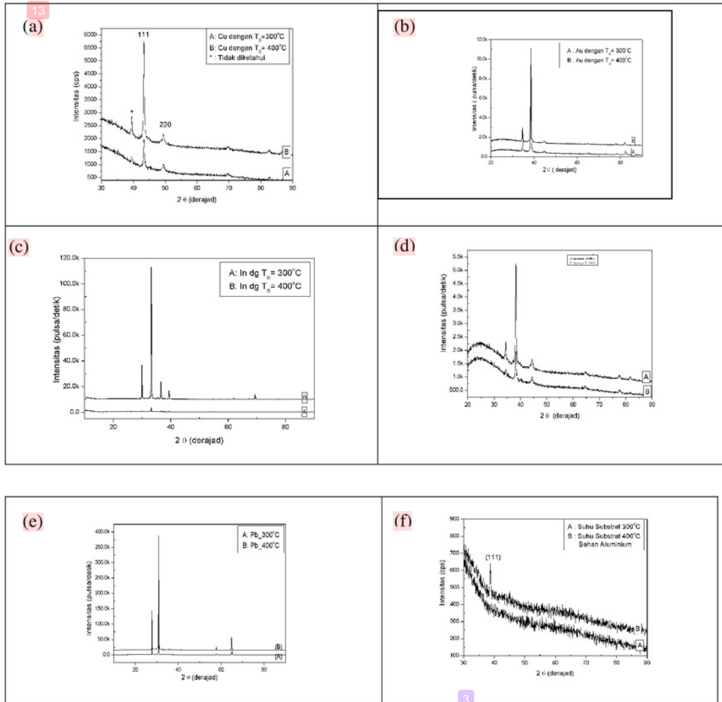
Gambar 1. Hasil XRD lapisan tipis: (a). Tembaga (Cu); (b). Emas (Au); (c). Indium (In); (d). Perak (Ag); (e). Timbal (Pb); dan (f). Aluminium (Al)
